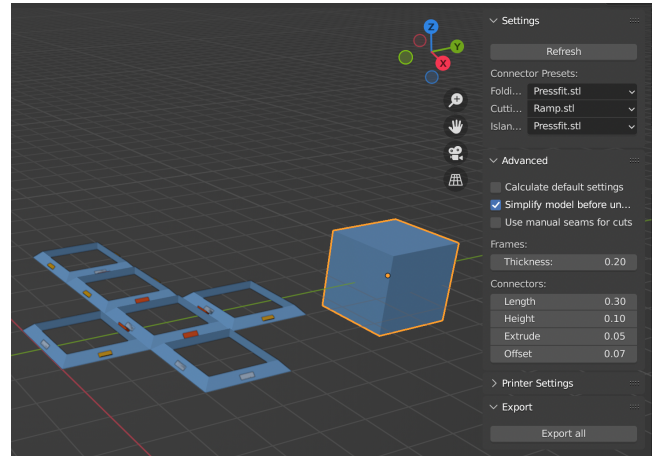
Figure 3: The interface of our plugin in Blender. The automatic process can be tuned manually via the Blender tool shelf on the right.
