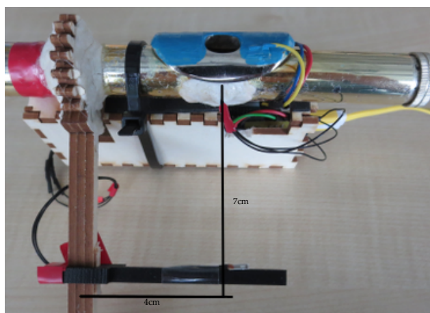
Figure 1: The sensor box attached to the head of a flute. The capacitive sensors for lip coverage are under the blue coating. The beam at the bottom of the image contains an air-flow sensor.
